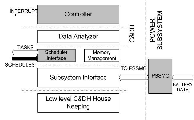
Figure 3 C&DH Architecture
